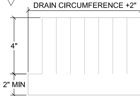
FLEX-FLASH F "SKIRT"
