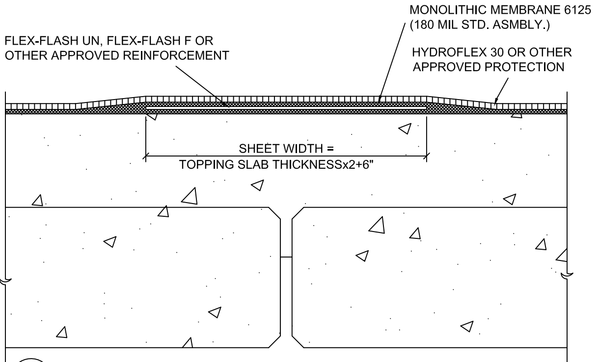
B NO SAW CUT
