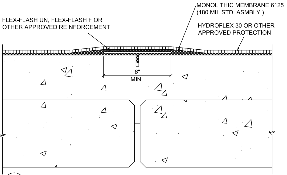
A SAW CUT TOPPING SLAB 1/4 SLAB THICKNESS
