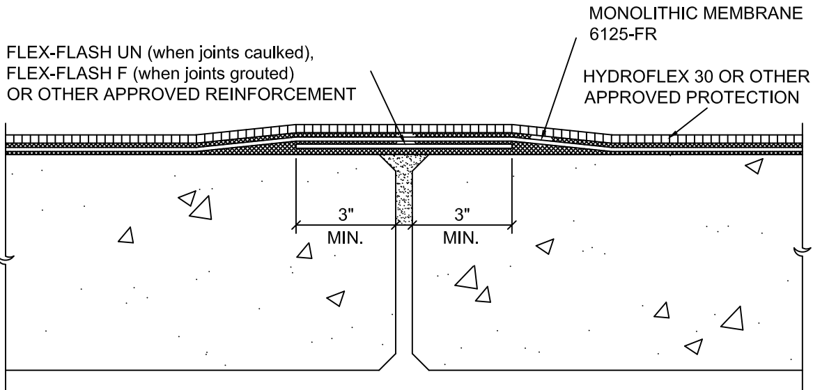
(A) WITHOUT TOPPING SLAB
