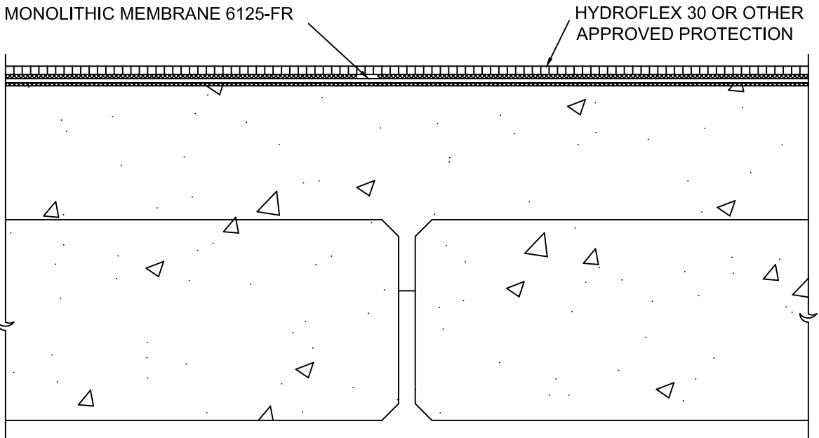
(B) WITH TOPPING SLAB
